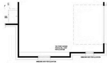
3RD CAR GARAGE OPT. "A"
