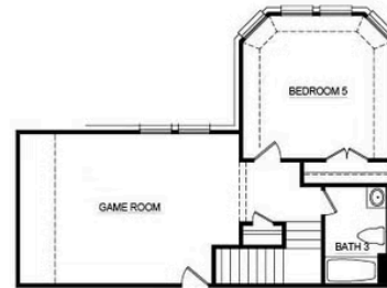
OPT. SECOND FLOOR BEDROOM #5 W-GAME ROOM
